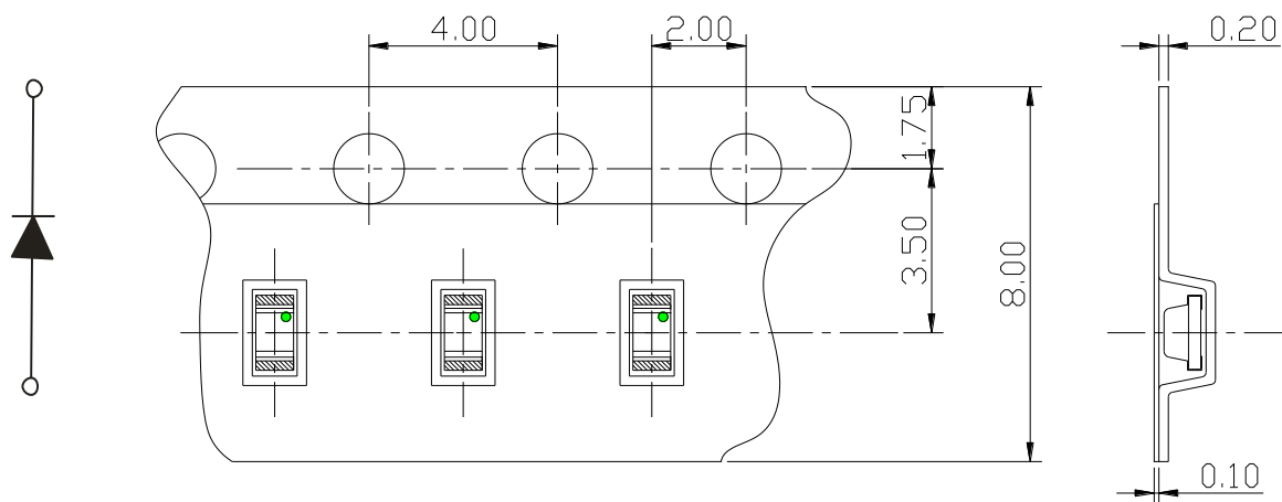
单位: mm, 未注公差: \pm 0.1 mm All dimensions in mm, tolerances unless mentioned is \pm 0.1 mm.
