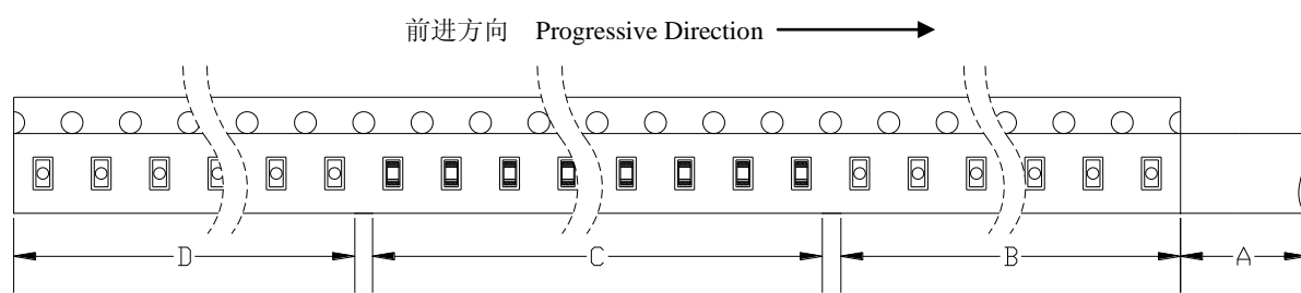
A: 盖带, 300 mm; B: 引导, 空带, 200mm; C: 编载产品 4000 只; D: 尾部, 空带, 200mm A: Top Cover Tape, 300mm; B: Leader, Empty, 200mm; C: 4000 Lamps Loaded; D: Trailer, Empty, 200mm.
